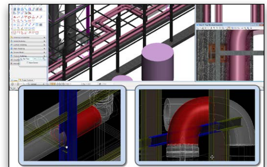
Hot-clash detection avoids costly operation failures and plant shutdowns.
