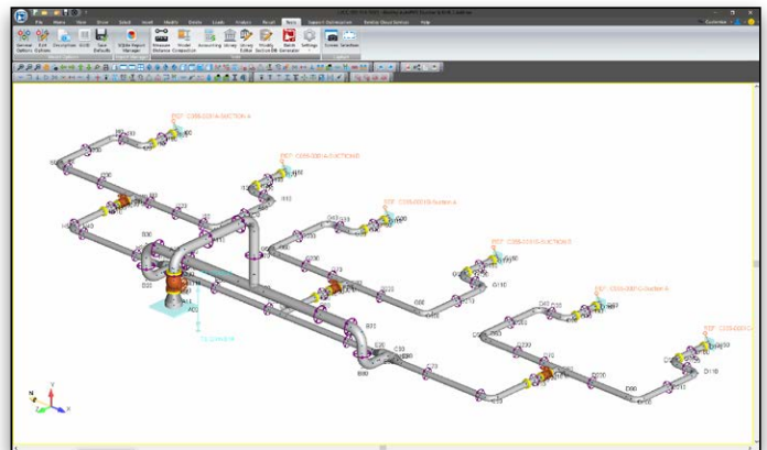
Determining the optimal arrangement for pipe supports automatically using Support Optimizer.
