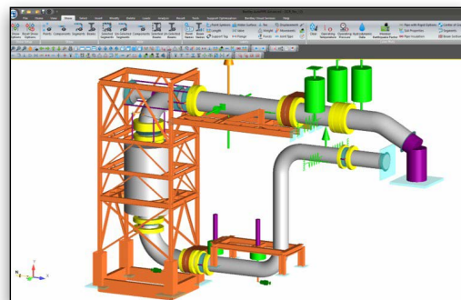
Pipe modeling using intuitive point-and-click graphical interface of AutoPIPE.
